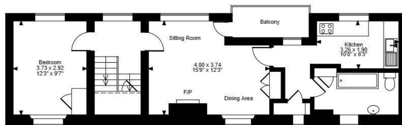
First Floor
