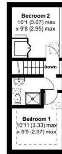
ANNEXE FIRST FLOOR
