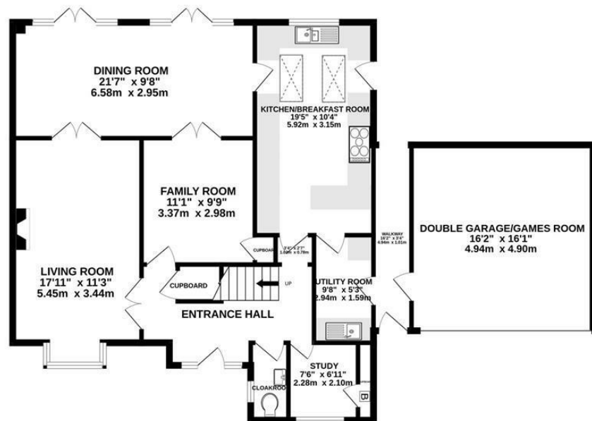
GROUND FLOOR 1280 sq.ft. (118.9 sq.m.) approx.
