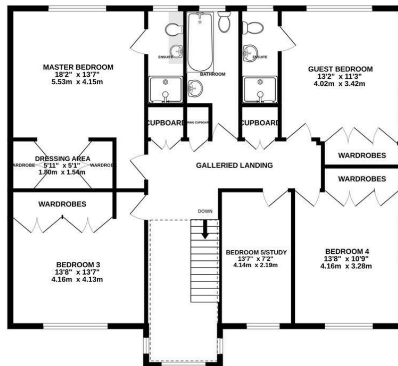
1ST FLOOR 1261 sq.ft. (117.2 sq.m.) approx.
