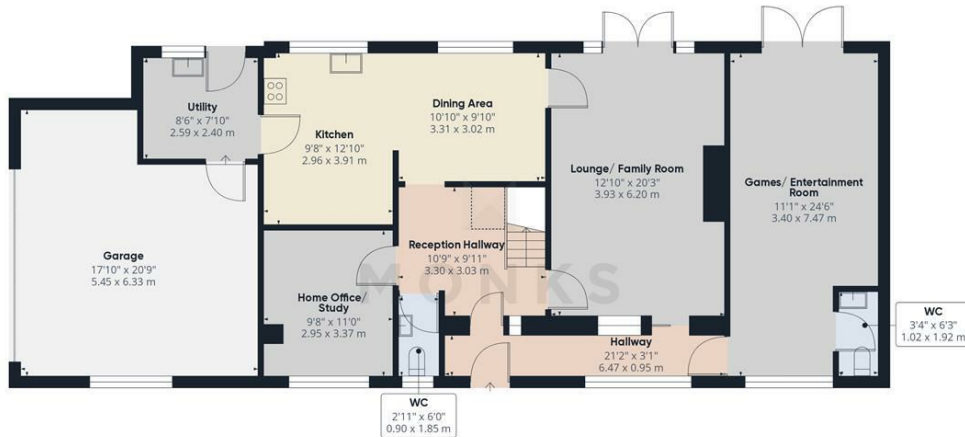
Floor 0
