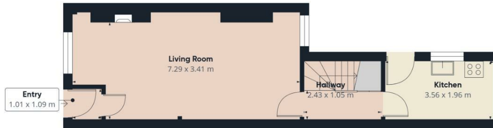
Ground Floor
