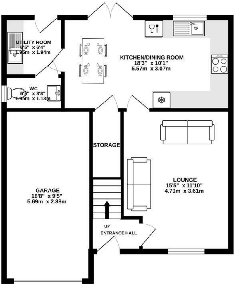
GROUND FLOOR 659 sq.ft. (61.3 sq.m.) approx.
