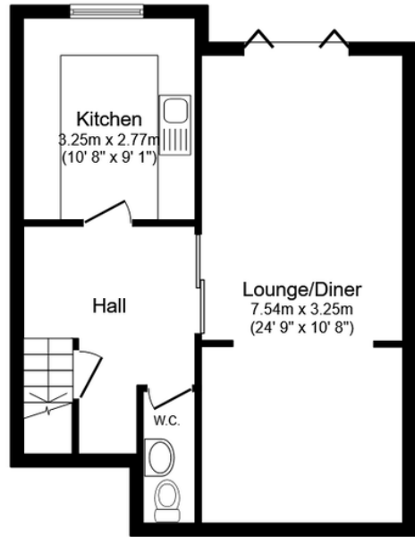
Ground Floor Floor area 45.7 m 2 (492 sq.ft.)
