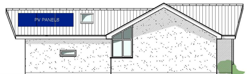
Proposed Side Elevation (East) scale 1:100
