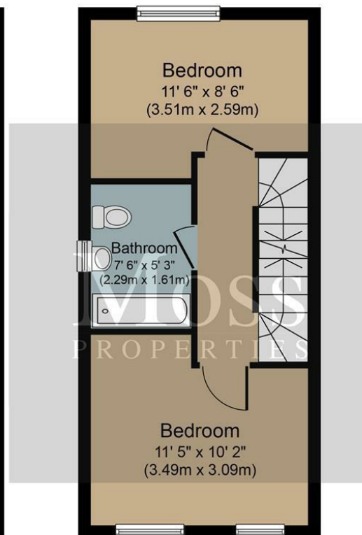
First Floor Approximate Floor Area 309 sq. ft. (28.7 sq. m.)
