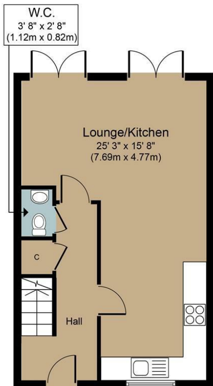
Ground Floor Approximate Floor Area 395 sq. ft. (36.7 sq. m.)
