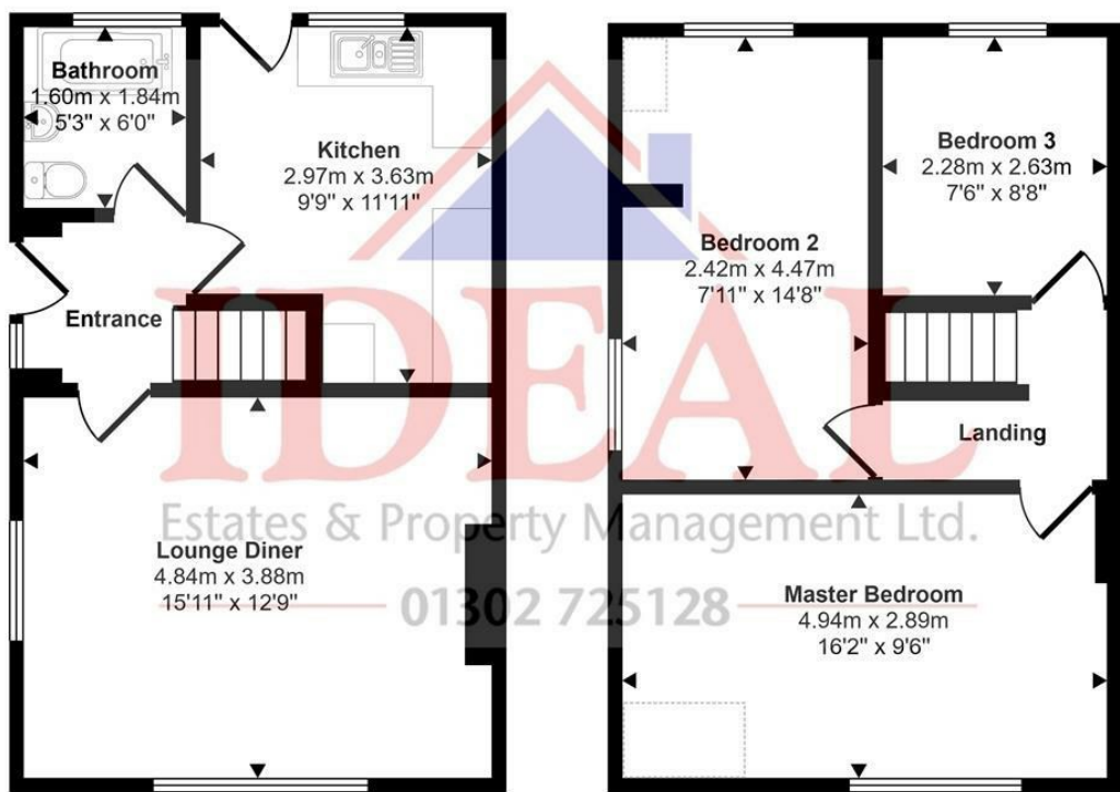
Ground Floor Approx 37 sq m / 394 sq ft
