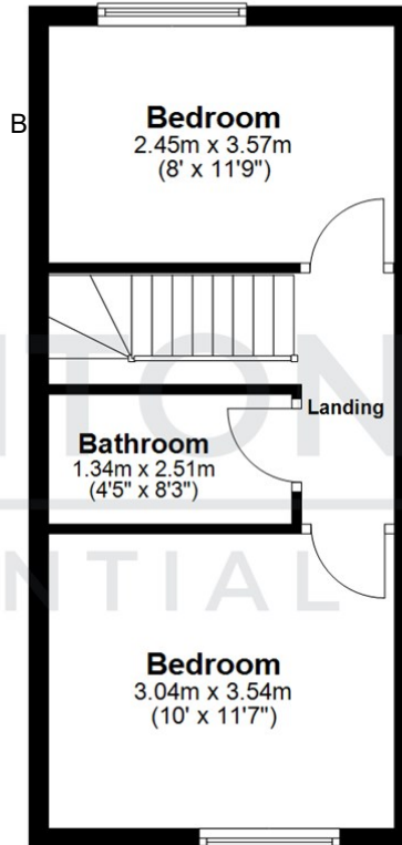
First Floor Approx. 29.5 sq. metres (317.2 sq. feet)
