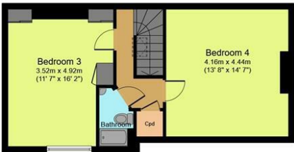
Second Floor
