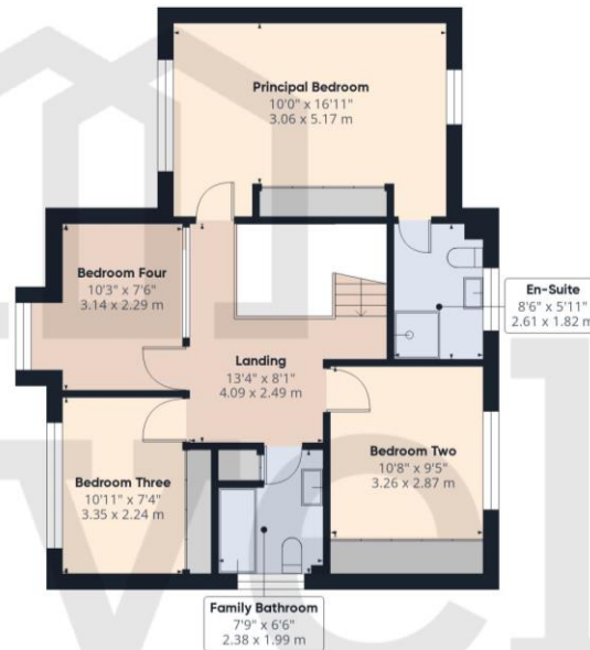
Floor 1 Building 1
