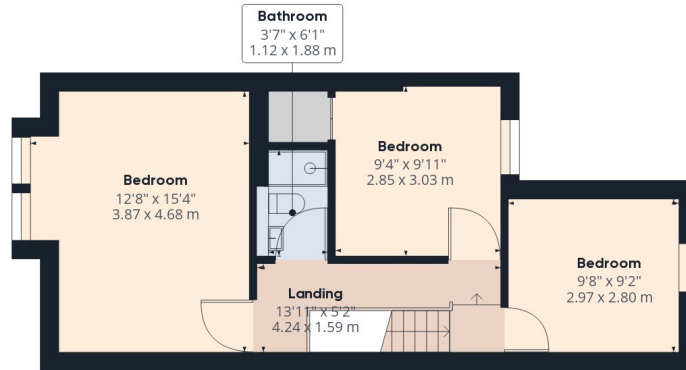
Floor 1 Building 1
