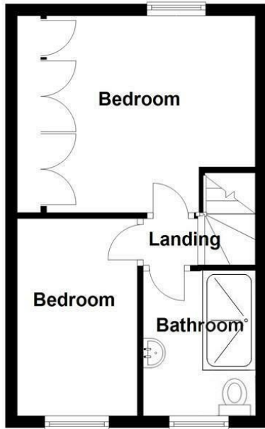
First Floor Approx. 26.2 sq. metres (281.5 sq. feet)
