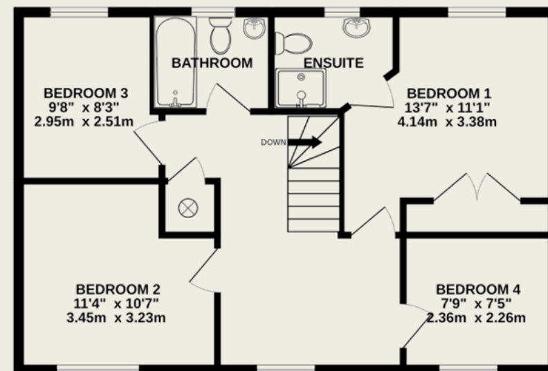
1ST FLOOR 619 sq.ft. (57.5 sq.m.) approx.
