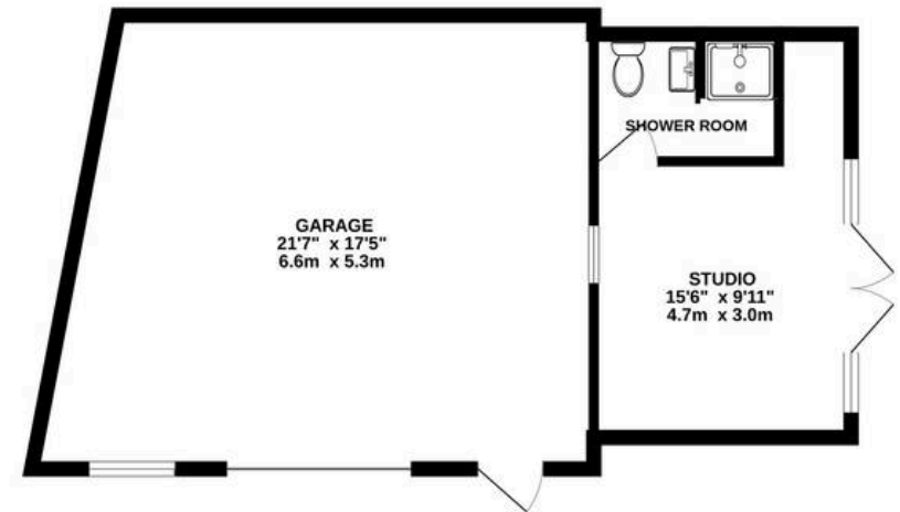
GARAGE & STUDIO 500 sq.ft. (46.4 sq.m.) approx.
