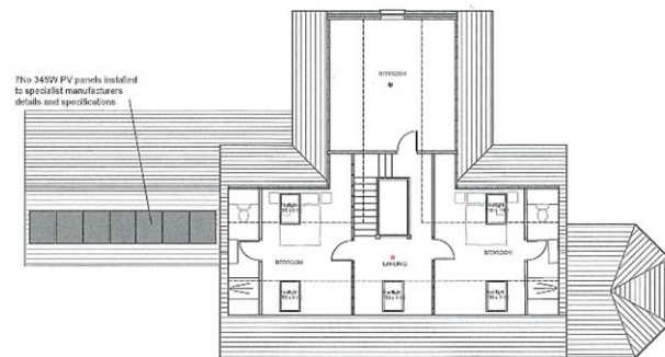
SECOND FLOOR PLAN - 1:100
