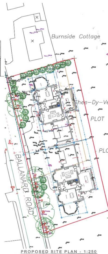
PROPOSED SITE PLAN - 1:250
