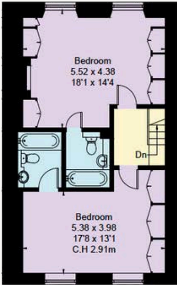
THIRD FLOOR
