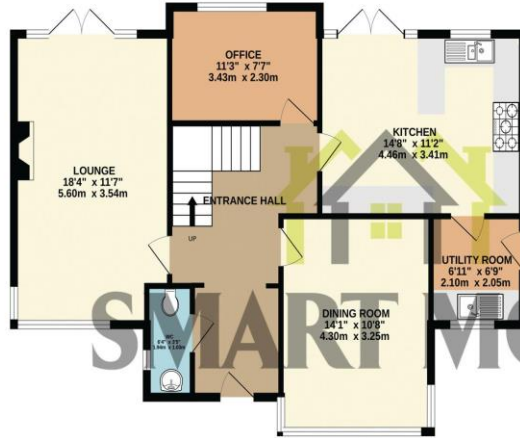
GROUND FLOOR 868 sq.ft. (80.7 sq.m.) approx.
