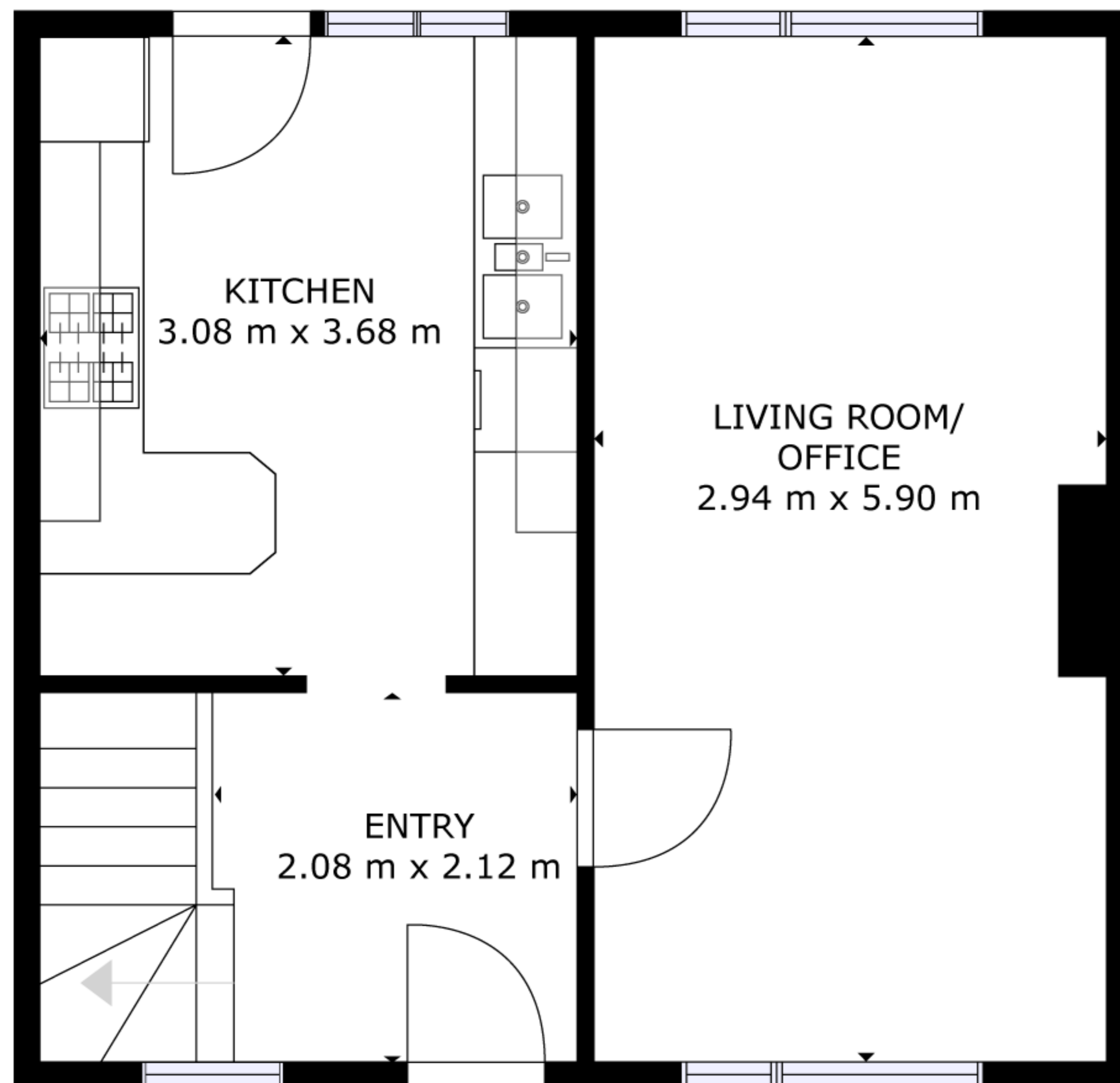
FLOOR 1
