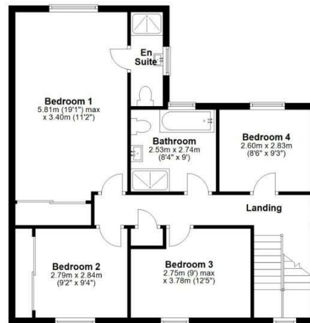
First Floor Approx. 72.5 sq. metres (780.3 sq. feet)
