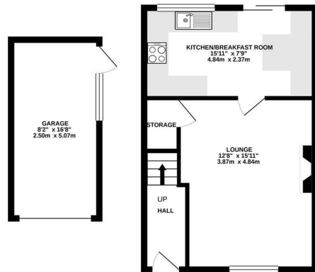
GROUND FLOOR 519 sq.ft. (48.2 sq.m.) approx.
