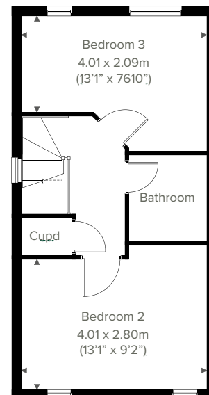
2ND FLOOR
