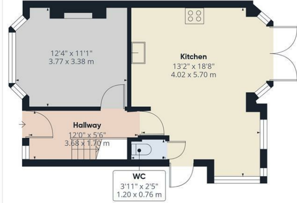
Floor 0 Building 1
