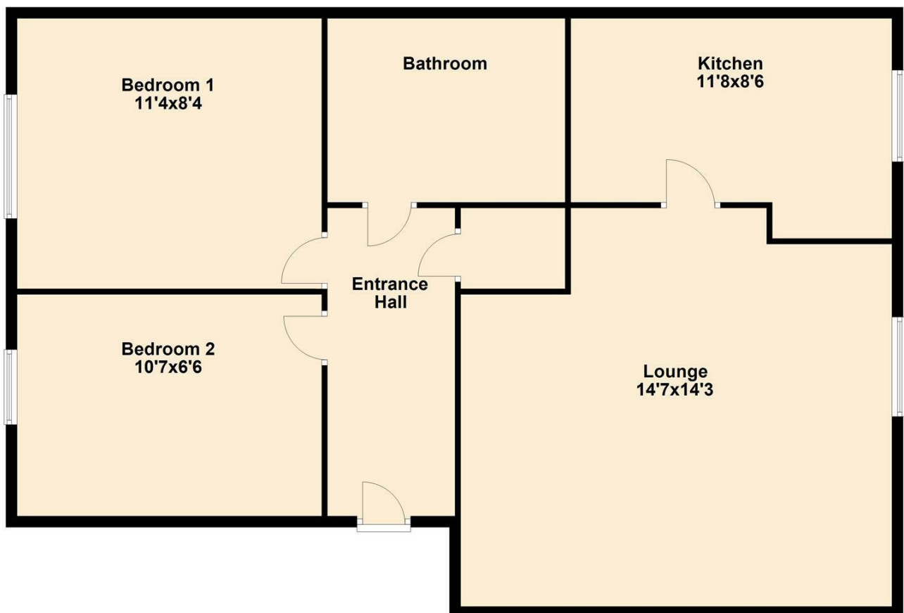
Floor Plan
