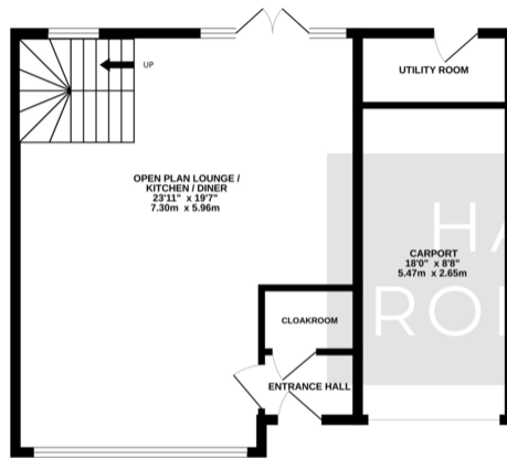
GROUND FLOOR 650 sq.ft. (60.4 sq.m.) approx.
