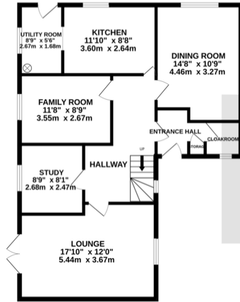
GROUND FLOOR 1139 sq.ft. (105.9 sq.m.) approx.
