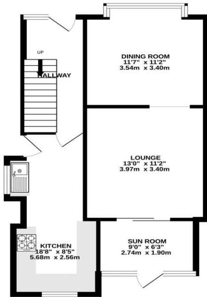
GROUND FLOOR 532 sq.ft. (49.5 sq.m.) approx.
