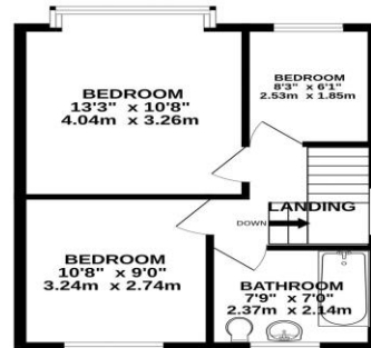
1ST FLOOR 389 sq.ft. (36.1 sq.m.) approx.
