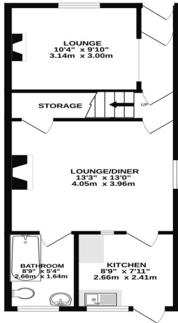
GROUND FLOOR 452 sq.ft. (42.0 sq.m.) approx.
