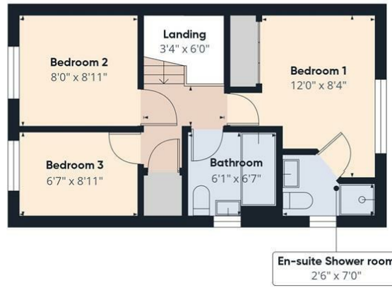
Floor 1 Building 1
