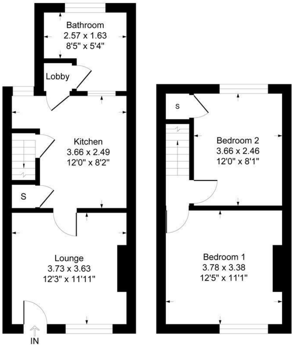
Ground Floor
