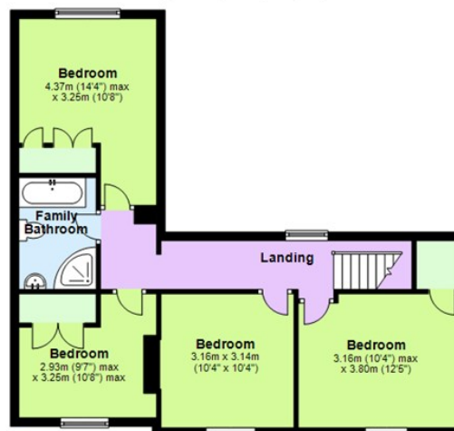
First Floor Approx. 62.3 sq. metres (670.1 sq. feet)
