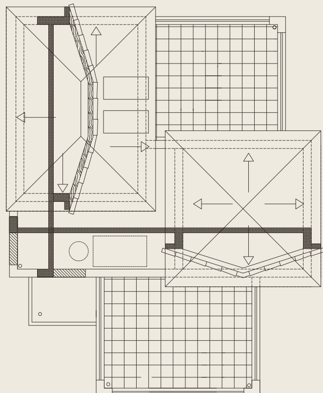
ROOF PLAN
