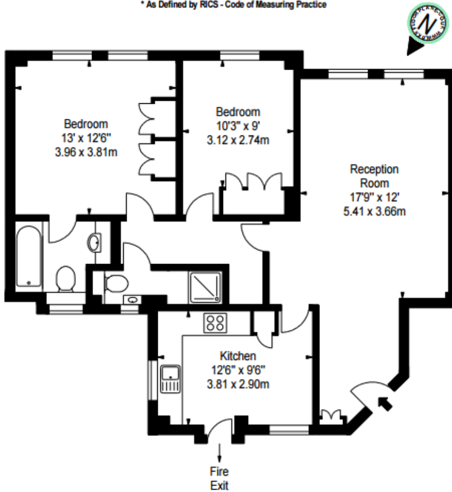
SECOND FLOOR
