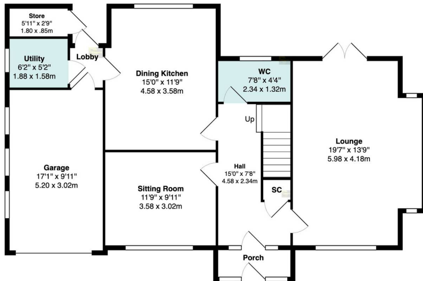
Ground Floor Approximate Area: 974 ft 2 ... 90.4 m 2
