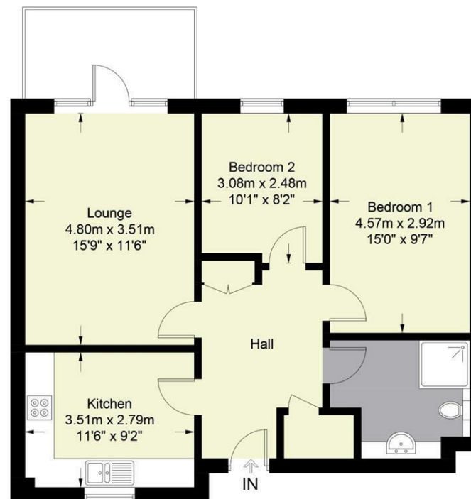
FOURTH FLOOR
