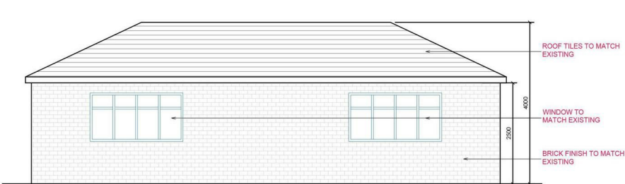
Proposed Annexe Left Side Elevation
