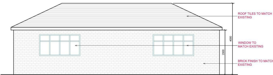
Proposed Annexe Right Side Elevation
