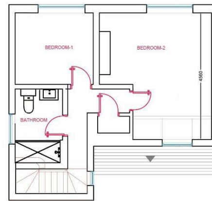
Existing First Floor
