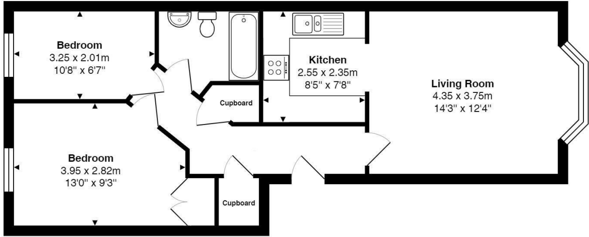
Ground Floor
