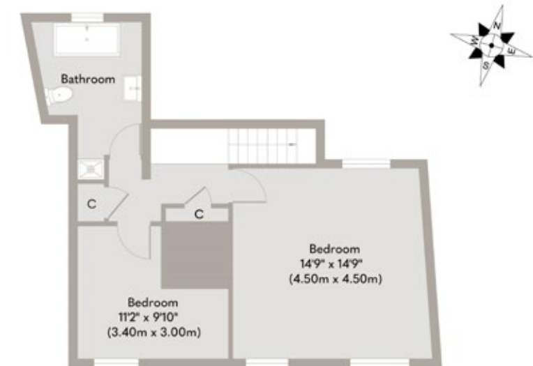
First Floor Approximate Floor Area 472 sq. ft (43.84 sq. m)
