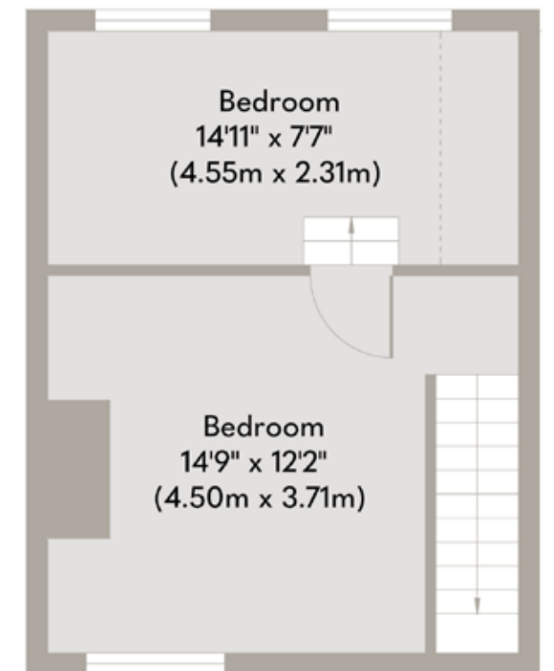
First Floor Approximate Floor Area 288 sq. ft (26.75 sq. m)
