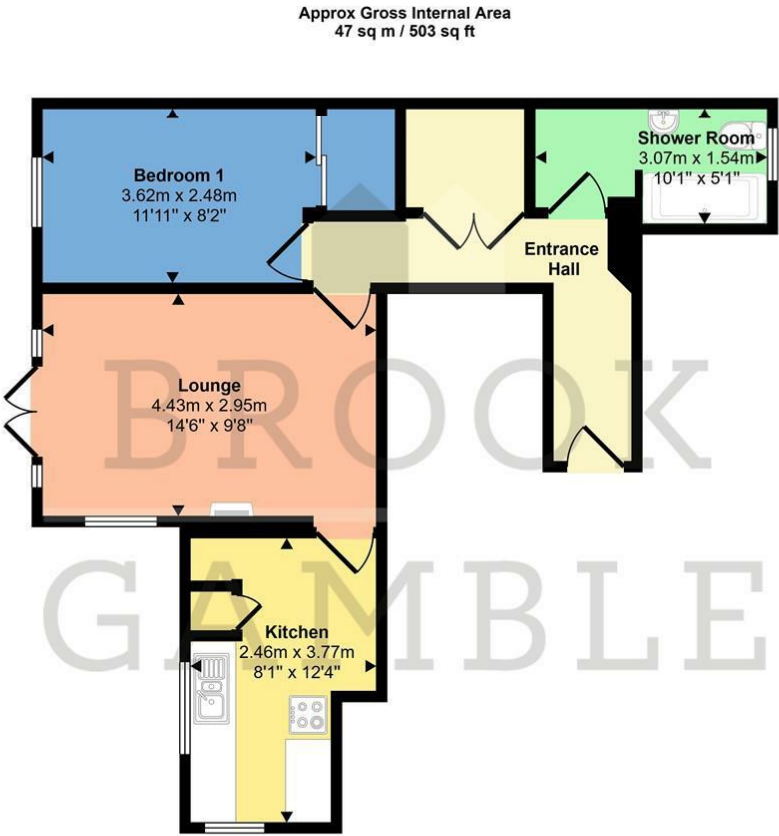
Floorplan
