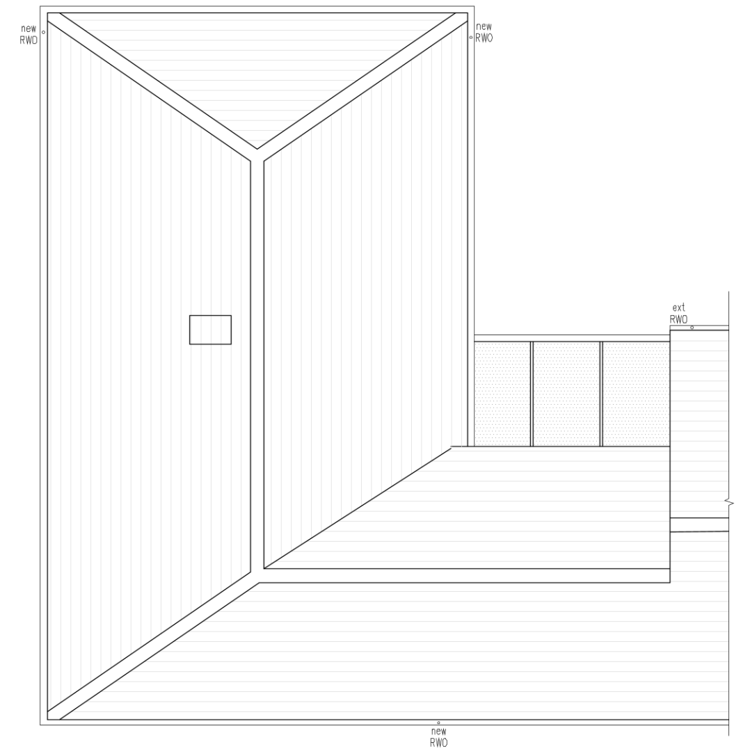
② Proposed Roof Plan.
