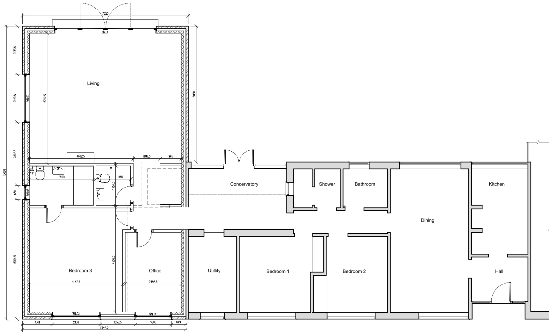
① Proposed Ground Floor Plan.
