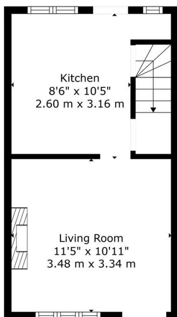
Floor 1
