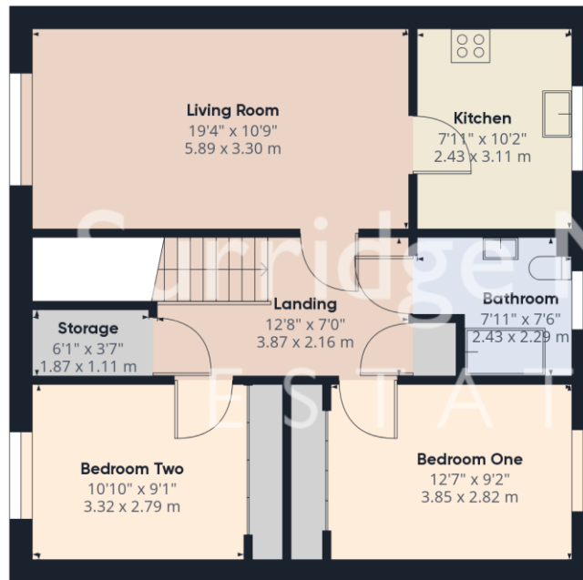
Floor 1
