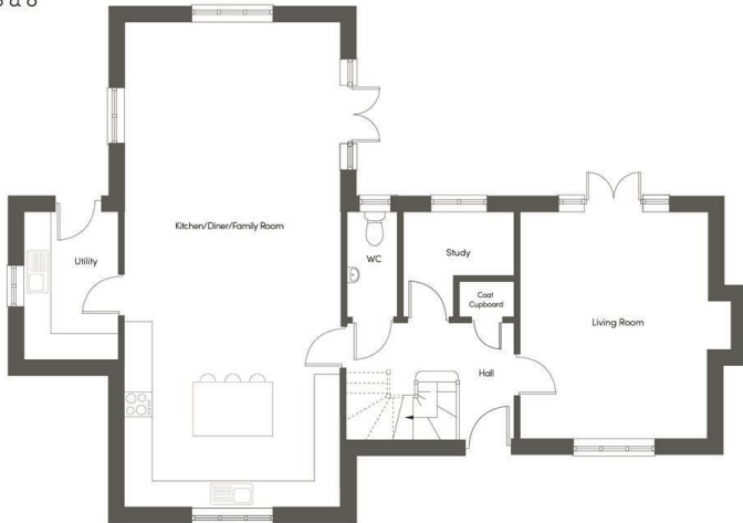
The Hampton Ground Floor Plots 1,3 & 8
