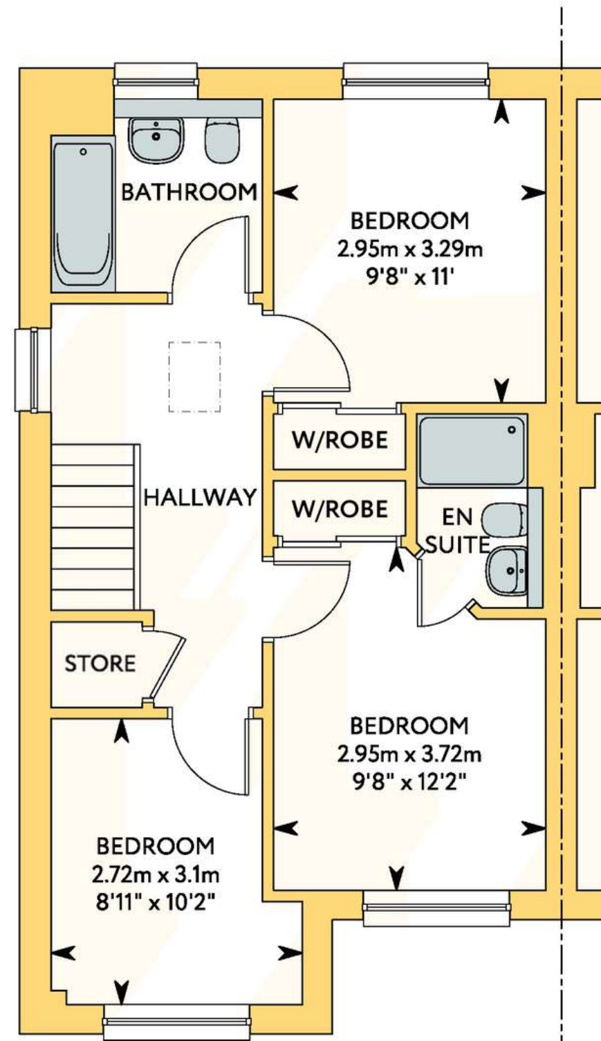
FIRST FLOOR
